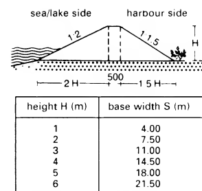
6 Mole or dam section (dimensions)
